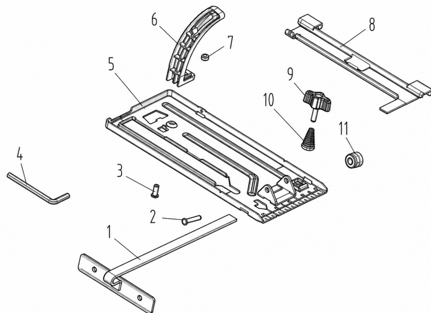
E - BASE PLATE GROUP
