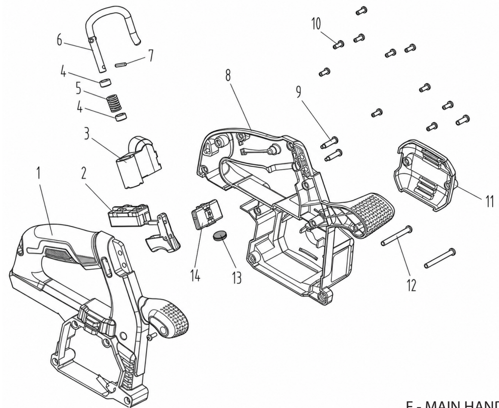
F - MAIN HANDLE ASSEMBLY GROUP
