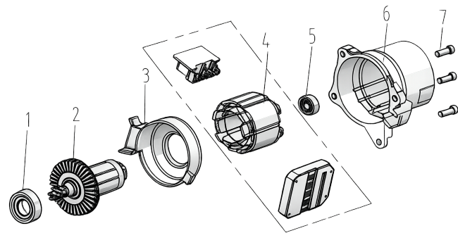
C - MOTOR ASSEMBLY GROUP
