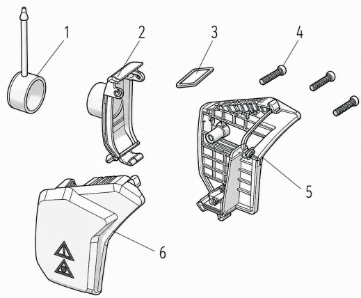
A - CHIP COLLECTOR GROUP
