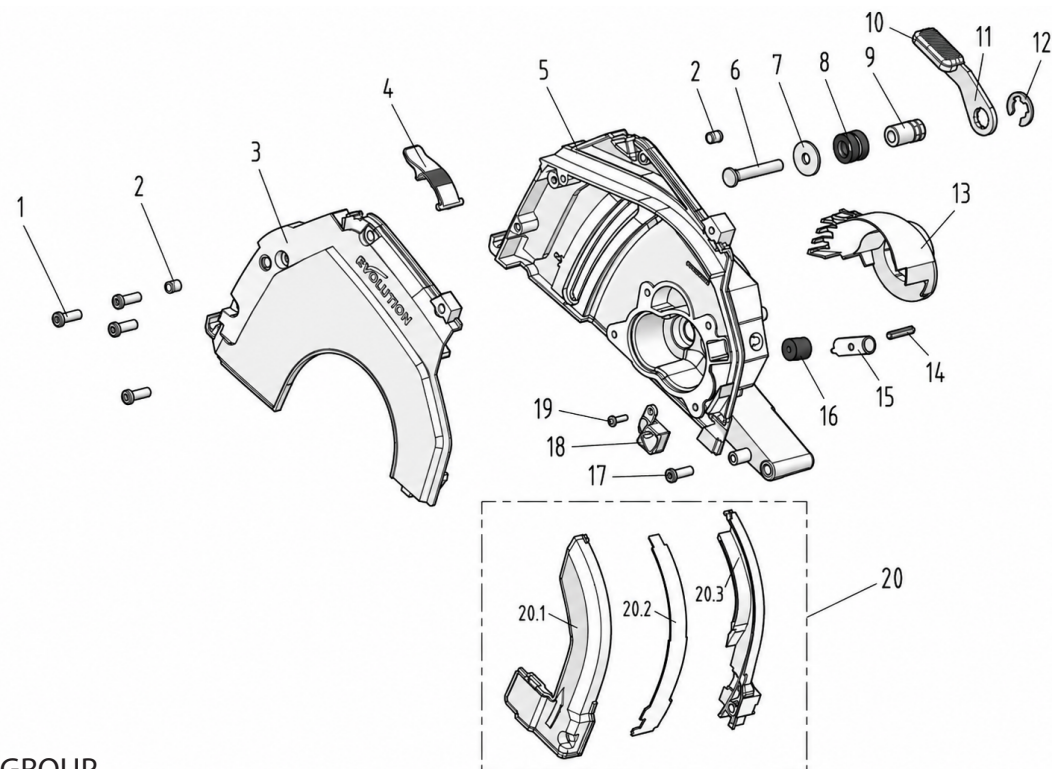
B - HEAD GROUP
